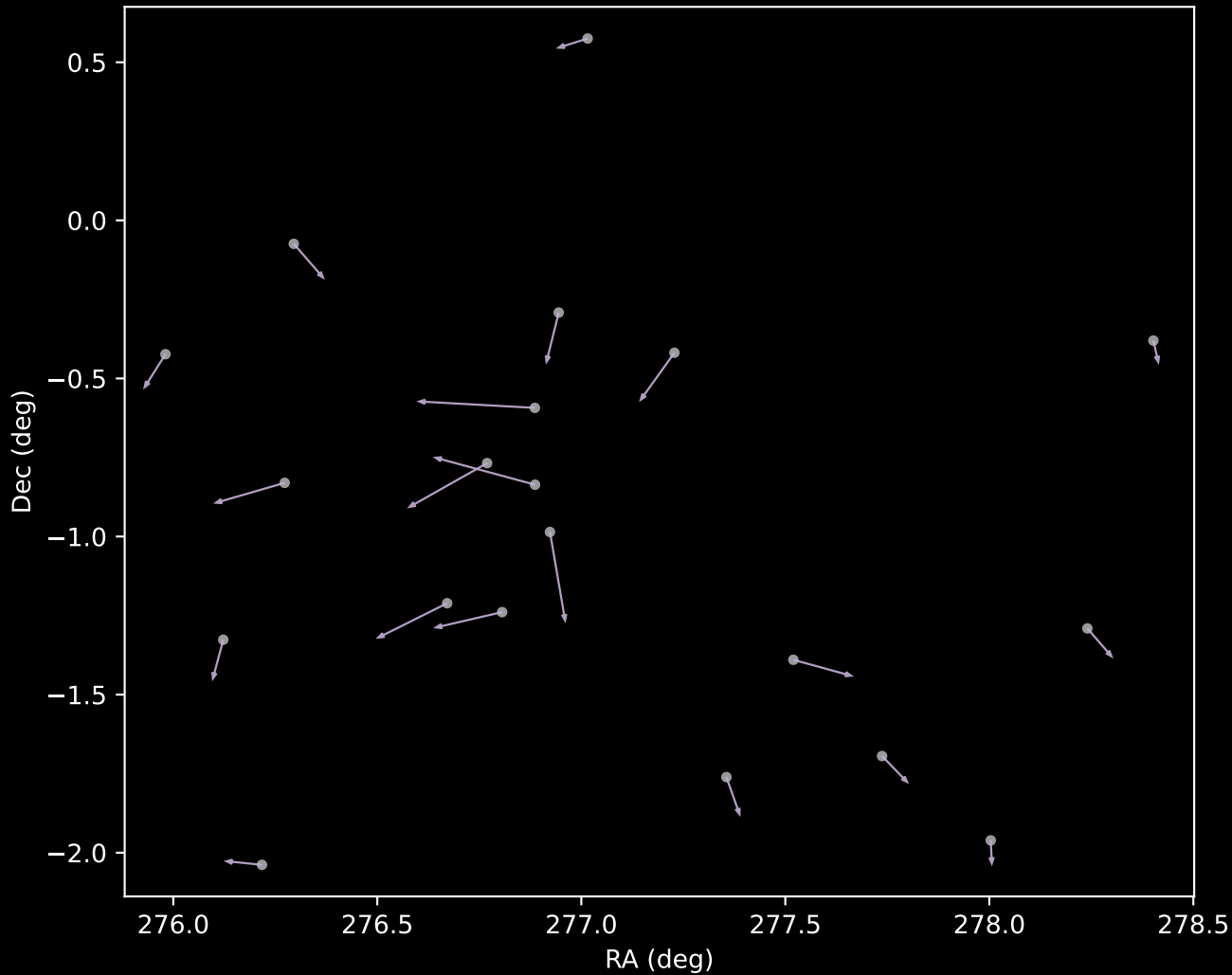
APOGEE DR17 Cluster 9 Proper Motion Vectors (n=20)
