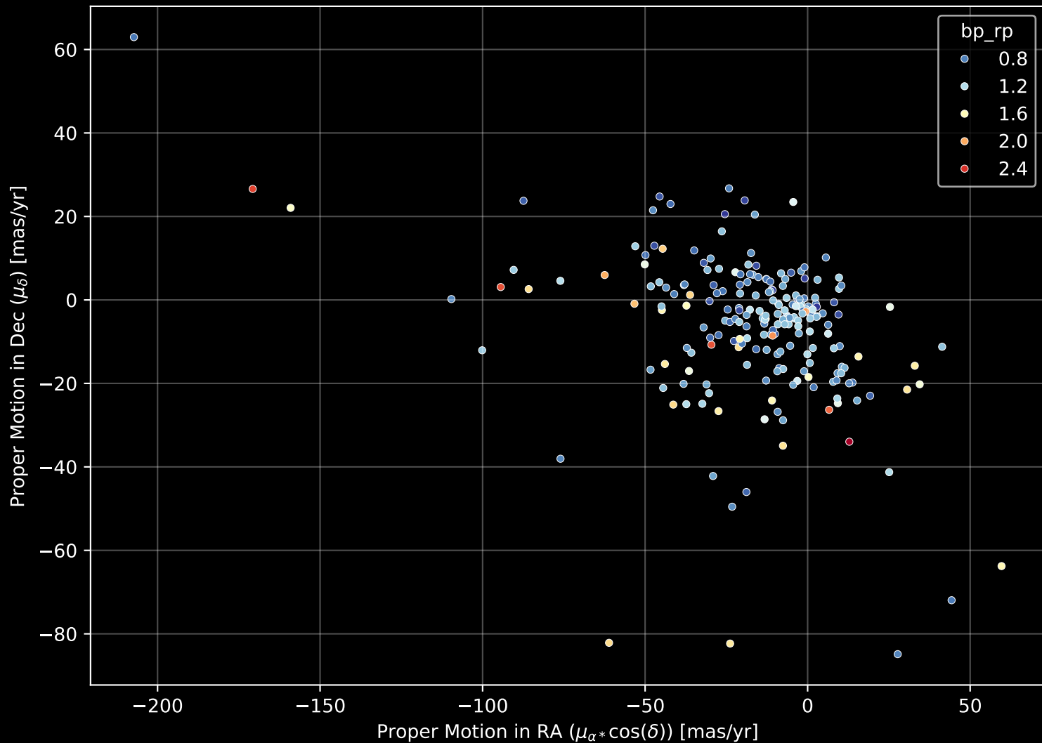
APOGEE DR17 Field: [272+58] Proper Motion Diagram (n= 222)
