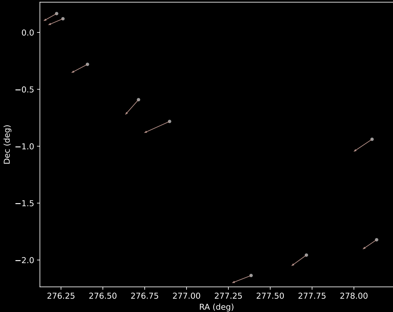
APOGEE DR17 Cluster 11 Proper Motion Vectors (n=9)
