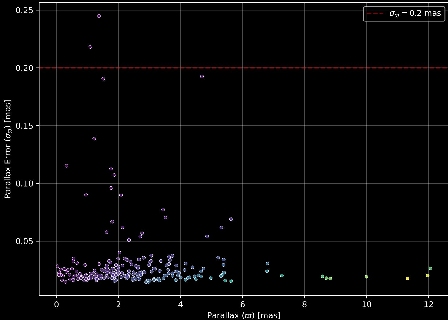
APOGEE DR17 Field: [272+58] Parallax Quality (n= 222)
