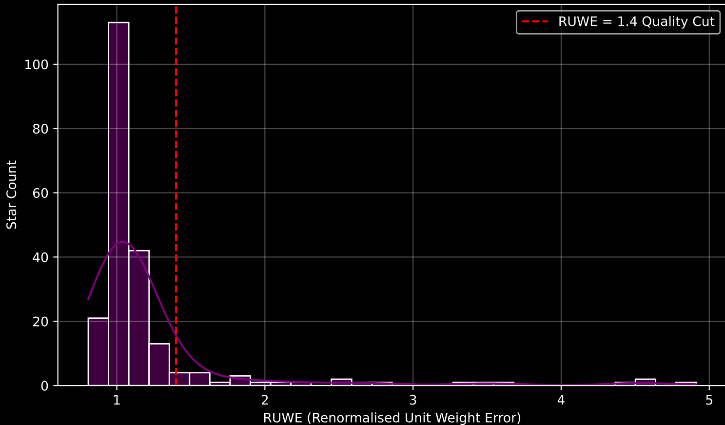
GAPOGEE DR17 Field [272+58] RUWE Distribution (n= 215)
