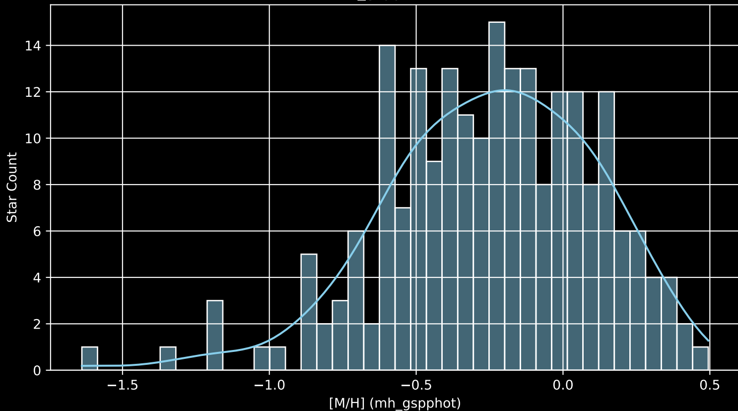
APOGEE DR17 Field: [272+58] [M/H] (mh_gspphot) (n= 218)
