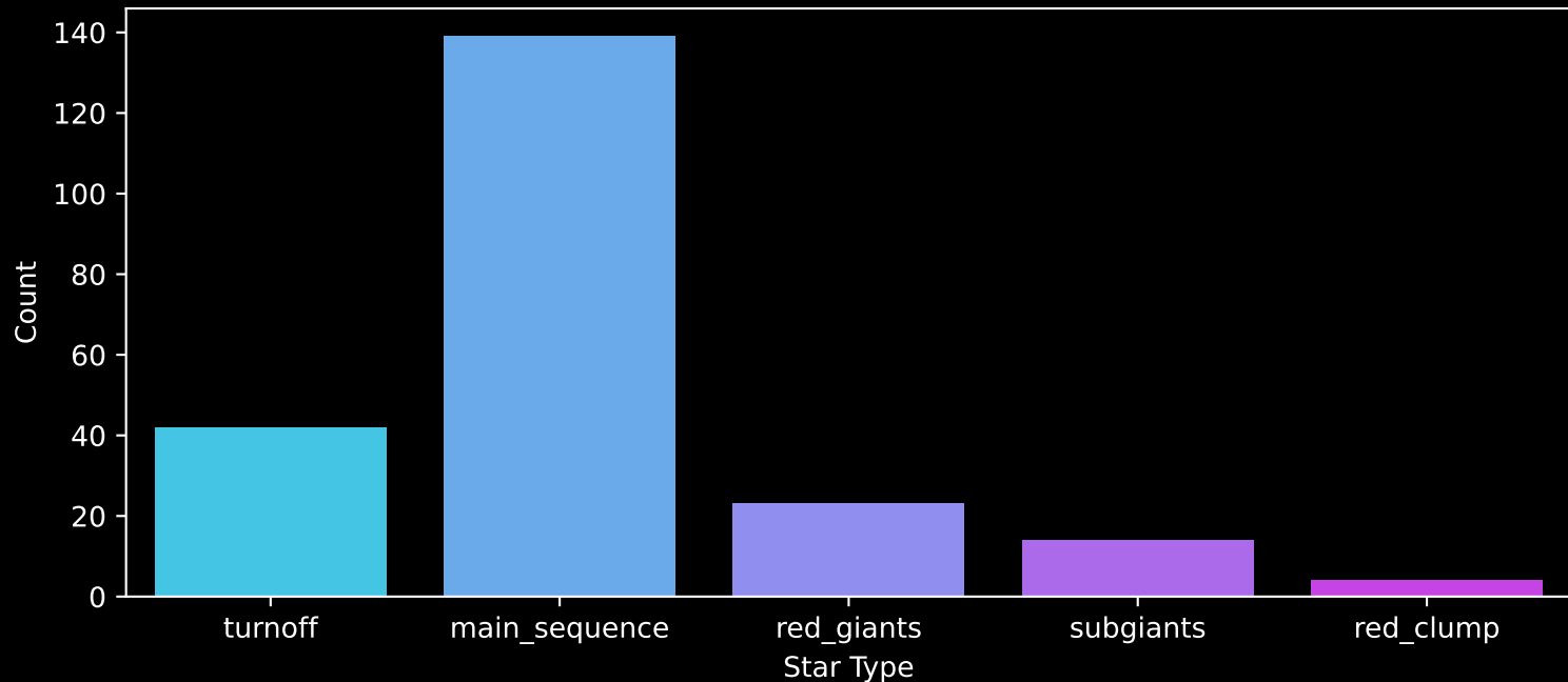
APOGEE DR17 Field: [272+58] Count plot of Star Type
