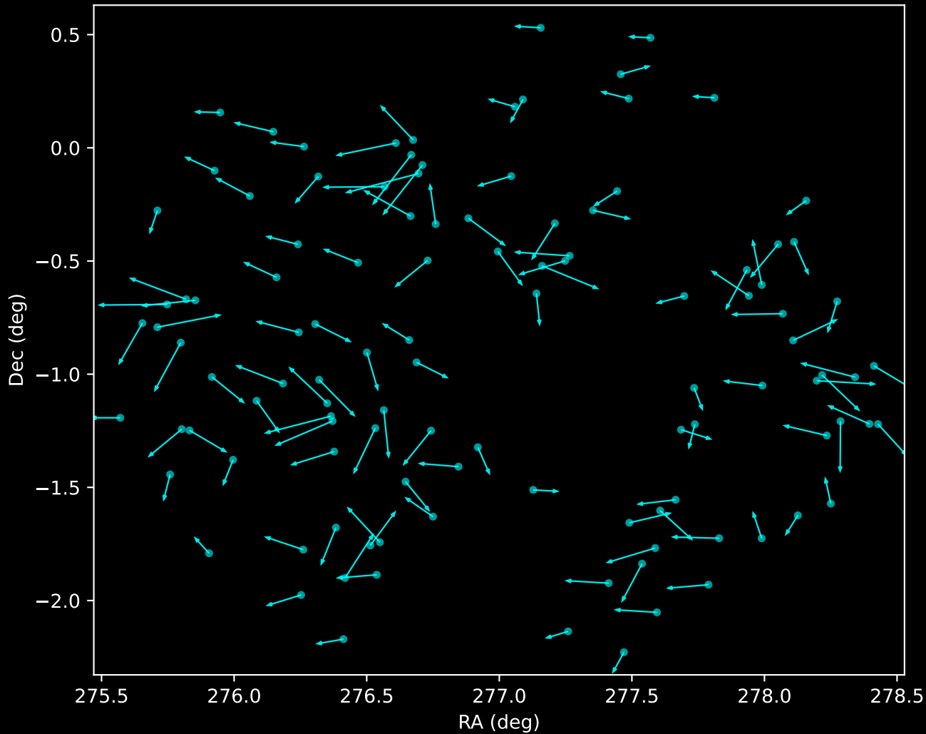
APOGEE DR17 Noise Stream Proper Motion Vectors (n=113)
